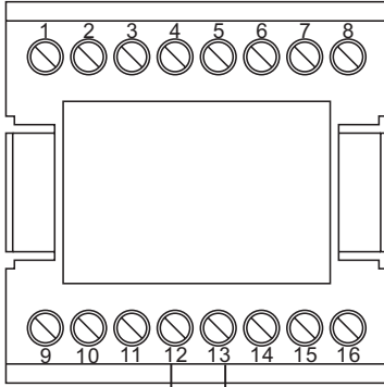
Figure 2.8 Input 1 Linear Current Wiring
