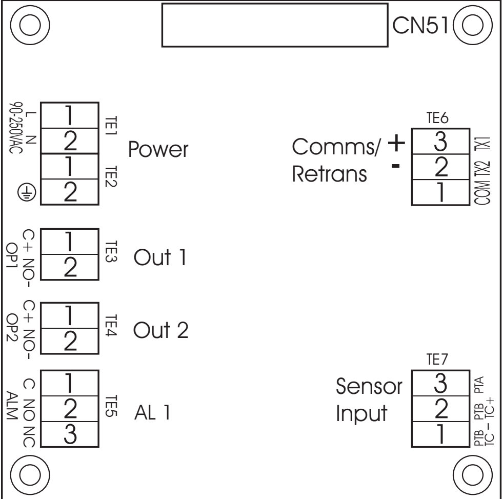
Figure 2.4 Terminal Connection
